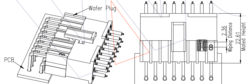
Plug:(R/A DIP TYPE)
