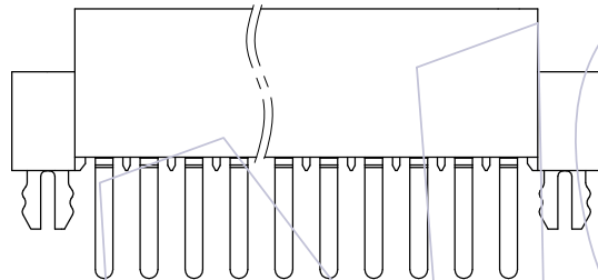
FIG. 2 WITHOUT NOTCH (SAME AS FIG.1, DIFFERENT AS SHOWN)
