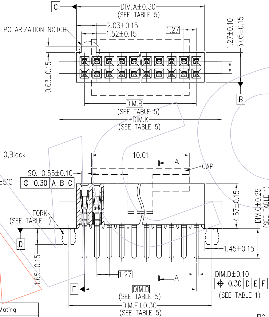
FIG. 1 THROUGH HOLE/STRAIGHT MODIFIED(-STD) LEAD STYLE: -01, -03
