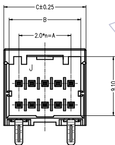
10P X-KEY
