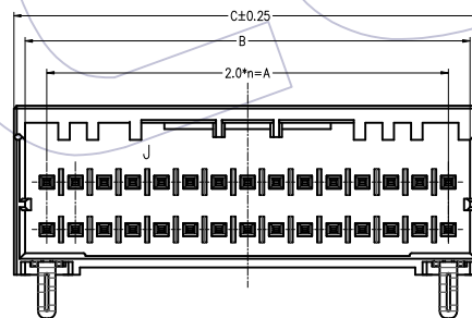
30P Y-KEY
