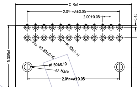
Recommended P.C.B Layout (Top Side) (PCB BOARD THICKNESS 1.0~1.6±0.05)
