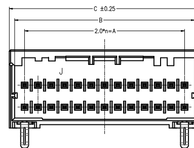
26P X-KEY
