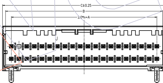
40P X-KEY
