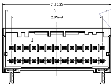
26P Y-KEY
