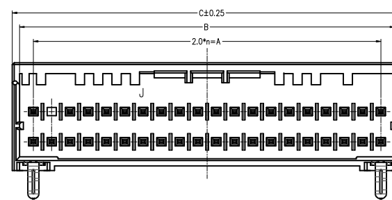
40P Y-KEY
