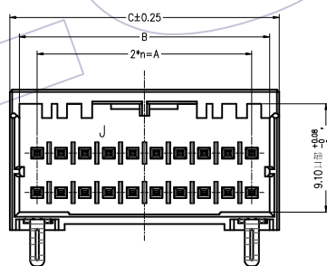
20P Y-KEY
