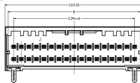
34P X-KEY
