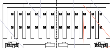
24PIN,X-KEY
