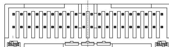
40PIN,Y-KEY
