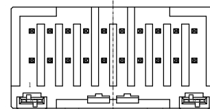
20PIN, X-KEY
