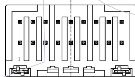
18PIN, X-KEY
