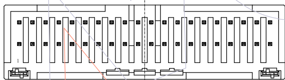
40PIN,X-KEY
