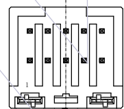
10PIN, X-KEY
