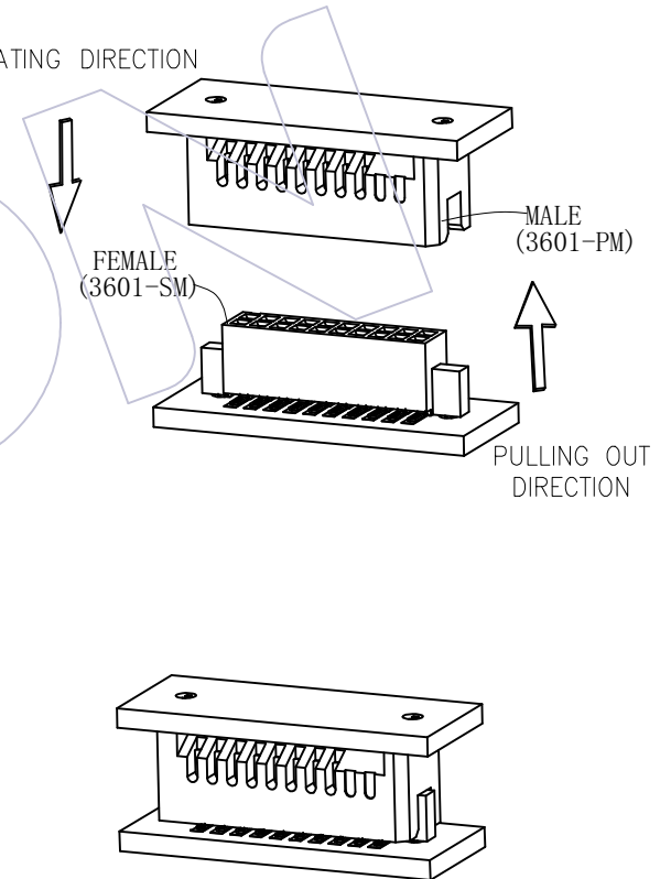
3601-PM MATED WITH 3601-SM
