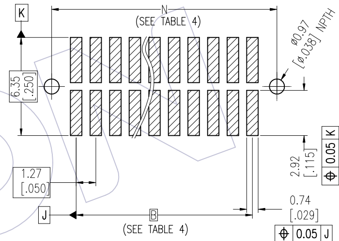
No. Pin Number (Per Row) POLARIZATION BUMP LOCKING A BUMP LOCKING B BUMP LOCKING C 3 2*5,2*7,2*8 NO YES NO NO 2 2*10-2*24 YES YES NO NO 2 2*25-2*34 YES YES YES NO 2 2*35-2*50 YES YES YES YES 1 2*10-2*50 YES NO NO NO 1 2*2-2*4,2*6 YES NO NO NO
