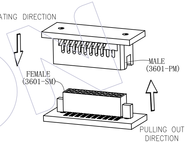
3601-PM MATED WITH 3601-SM
