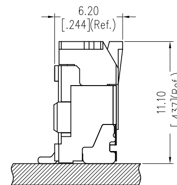
ASSEMBLY
